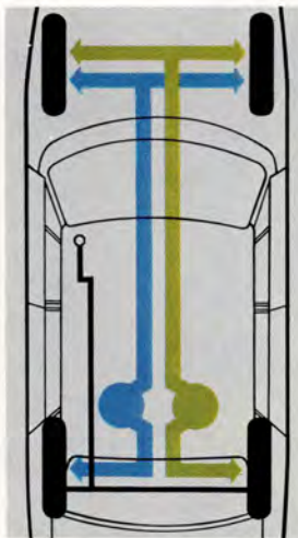
Braking system The 164's 4-wheel power disc braking system is really two separate systems. So if one system should ever fail the other is there to stop the car. Instead of having one system on the front wheels and another working on the rear wheels as on most cars, each Volvo braking system operates on three wheels—two front and one rear. The difference in braking efficiency is this. With the conventional front-and-rear split systems, the front wheels supply 70% of a car's braking and the rear wheels 30%. So if the front-wheel system should fail, you only have 30% of the braking power left to stop the car. But on the 164 where two fronts and one rear wheel always work together (in each system), braking efficiency is never less than 80%.
