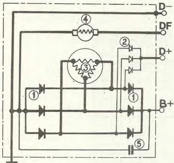
Generators inre koppling
