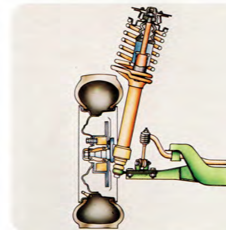
Cross-section showing the McPherson strut suspension.
