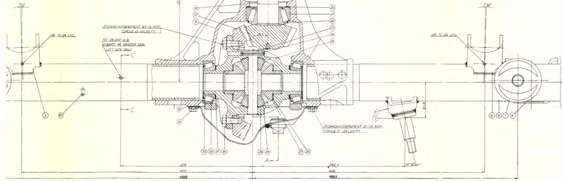
Genomskärningsritning, bakaxel 1031 Cut-away drawing, rear axle 1031
