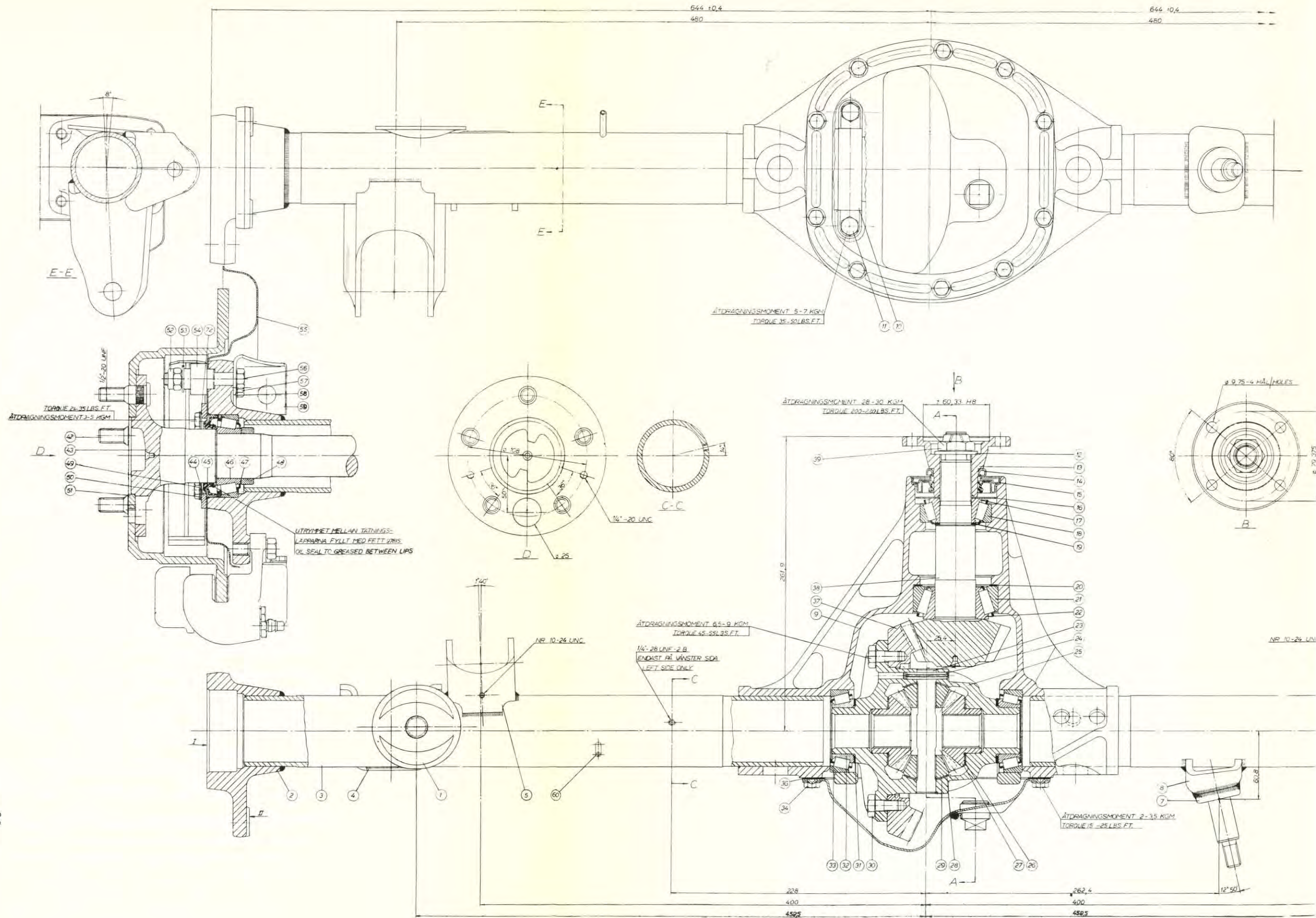
Genomsärningsritning, bakaxel 1031 Cut-away drawing, rear axle 1031
