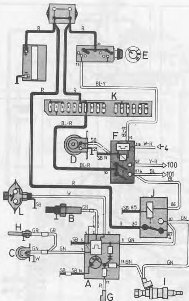
Engine running Frequency valve disengaged
