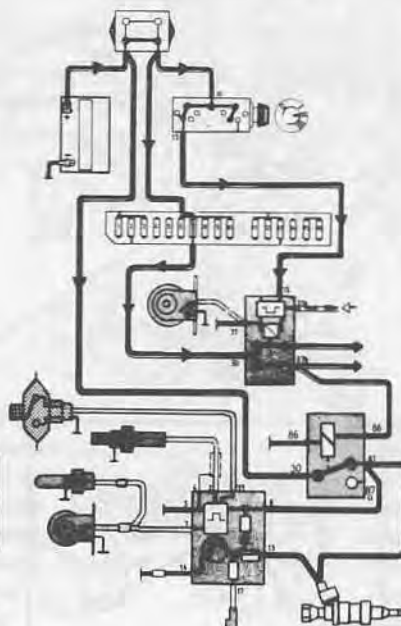
Engine running Frequency valve engaged
