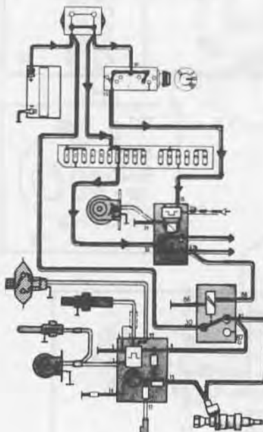
Engine running Frequency valve disengaged
